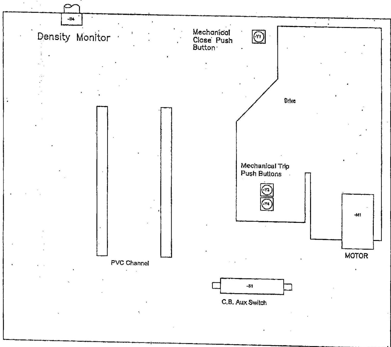
EQUIPMENT LAYOUT-REAR
