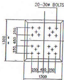
VIEW 3-3
