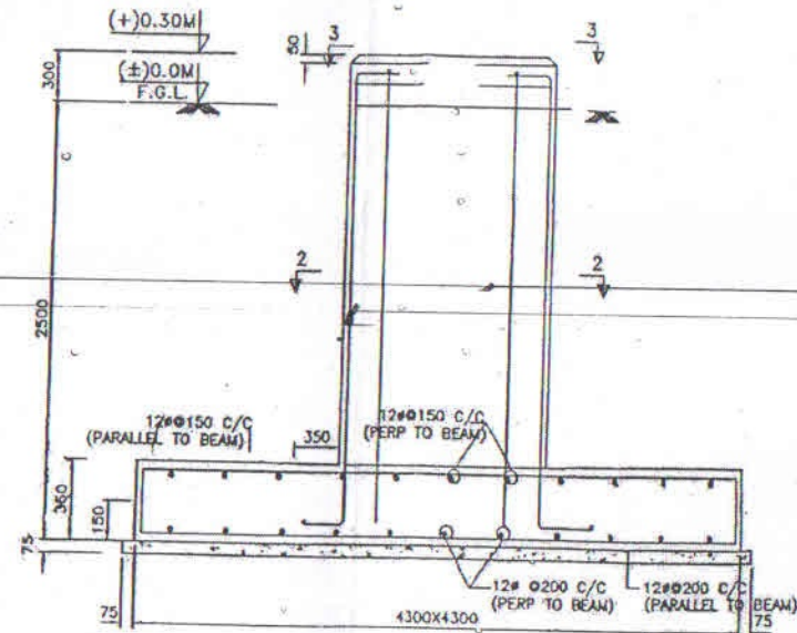
SECTION 1-1
