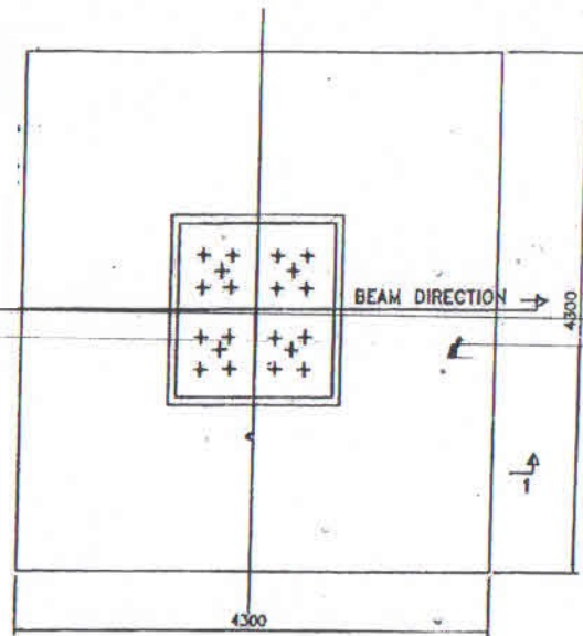
FOUNDATION PLAN
