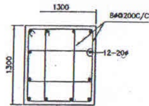
SECTION 2-2
