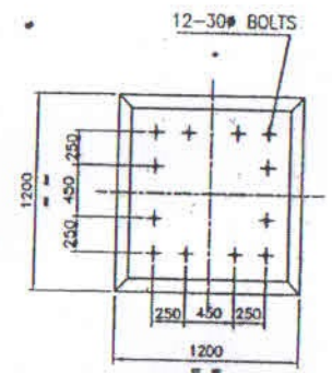
VIEW 3-3
