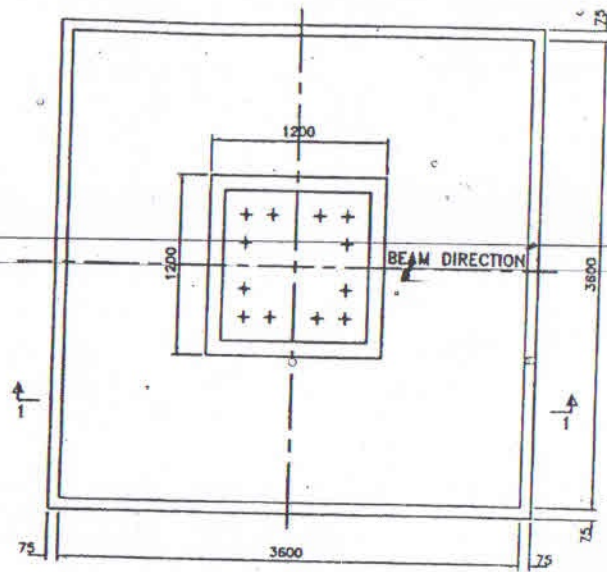
FOUNDATION PLAN
