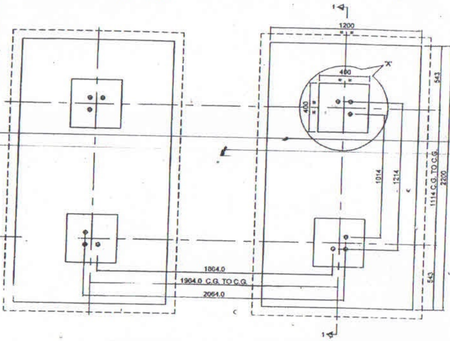
TYP. FOUNDATION PLAN FOR A-FRAME (A3)
