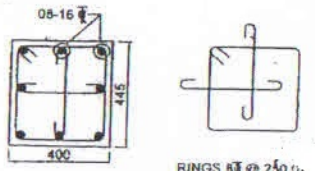
SECTION 2-2
