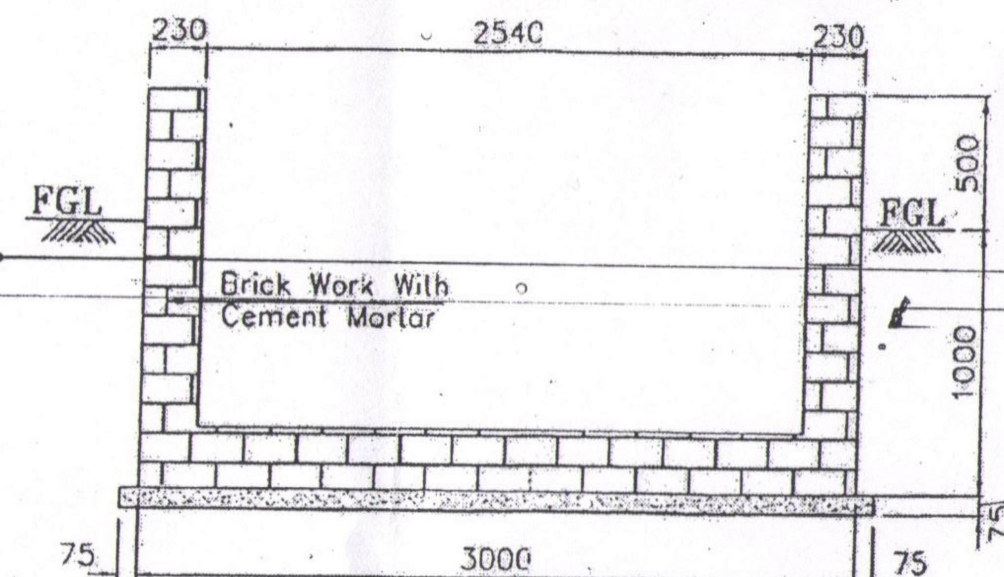
SECTION B-B
