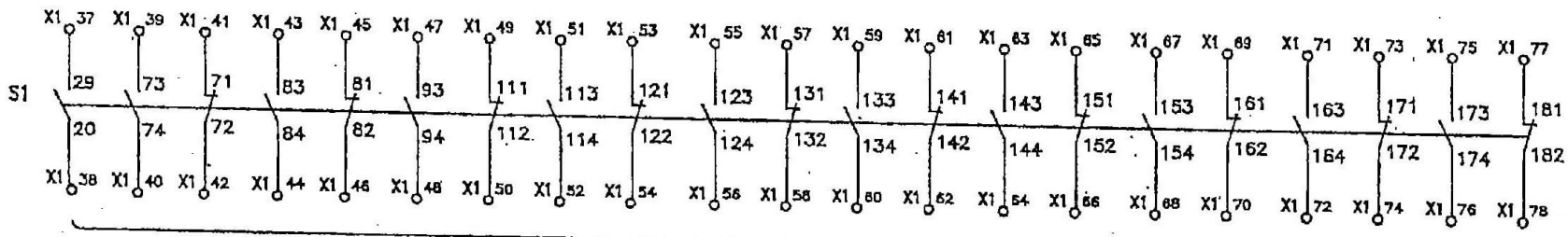
SPARE 10 NO / 10 NC CONTACTS OF CIRCUIT BREAKER AUX. SWITCH
