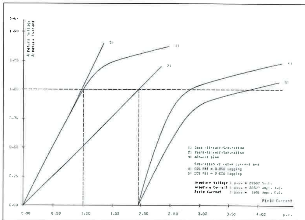
Figure 4: Saturation curve of generator.
